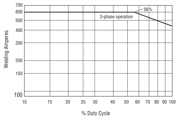
AlumaPower 450 MPa Duty Cycle Chart
