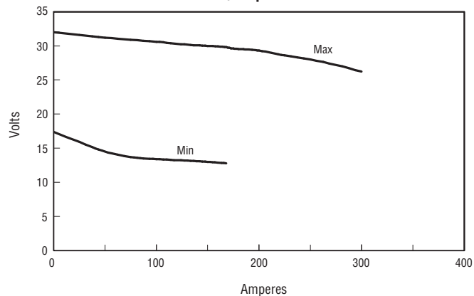
Volt/Amp Curves
