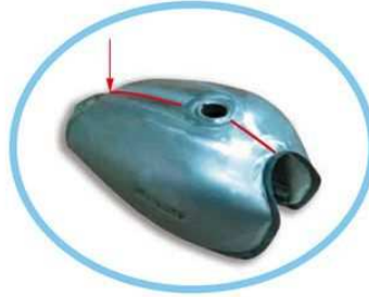
Horizontal Seam Welder for Longitudinal of Motorcycle Fuel Tank 摩托車油箱直線輪焊機
