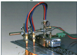
YK-450 / Elephant
