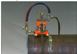
YK-20 / Phoenix
